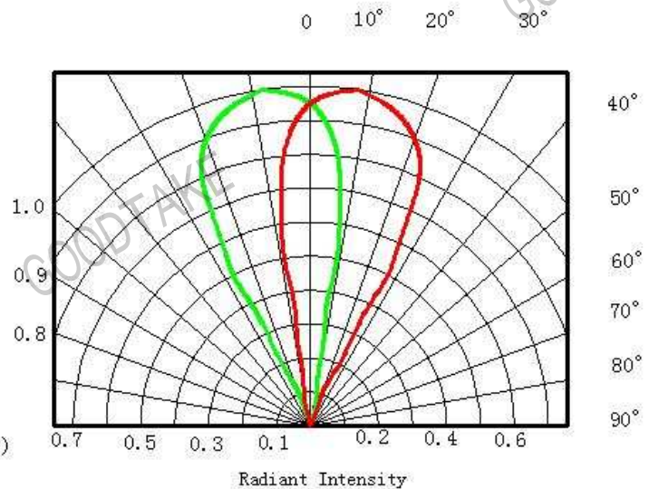
Fig.4 Angle Vs Radiant Intensity
