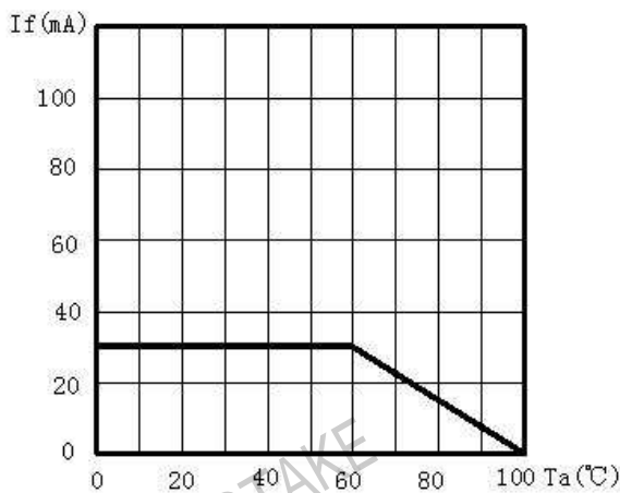
Fig. 3 Maximum Forward Current Vs Ambient Temperature
