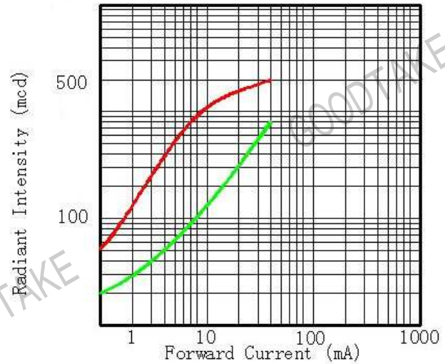
Fig. 2 Forward Current Vs Radiant Intensity
