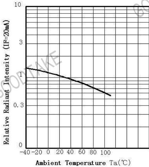
Fig.3 Ambient Radiant Intensity Vs Ambient Temperature
