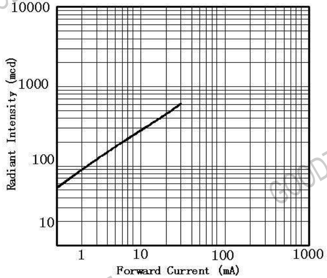
Fig.4 Forward Current Vs Radiant Intensity
