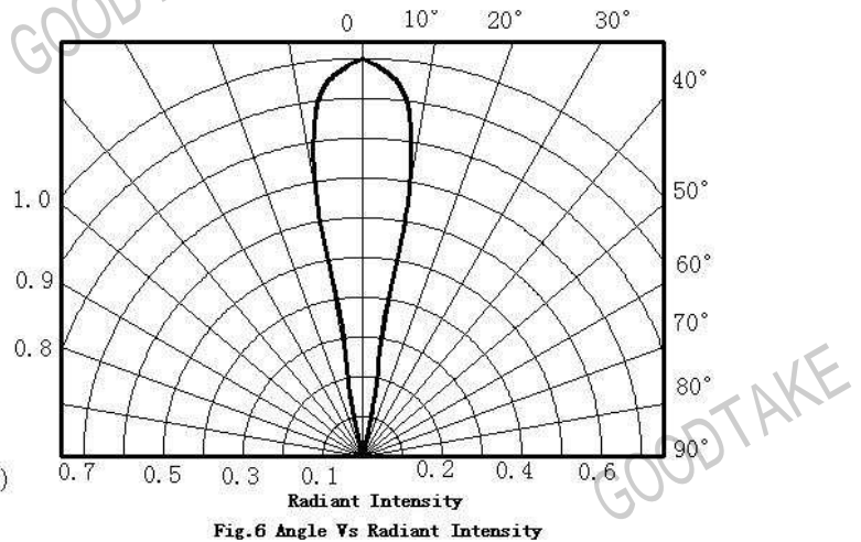
Fig.6 Angle Vs Radiant Intensity
