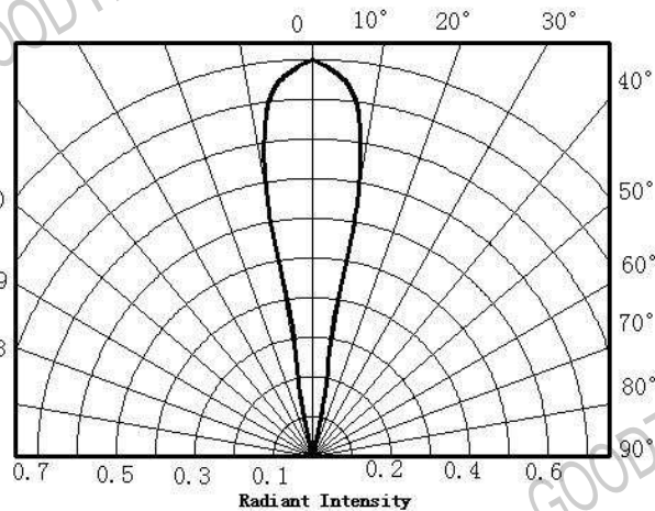
Fig.6 Angle Vs Radiant Intensity
