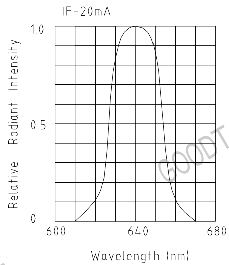
Fig.2 Spectral Distribution
