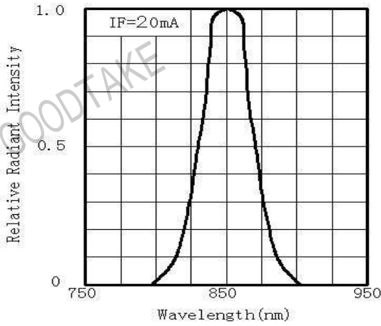
Fig.1 Spectral Distribution
