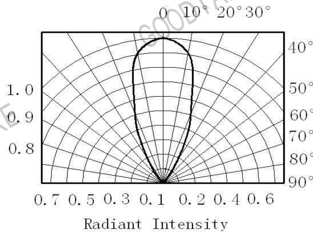
Fig.5 Angle Vs Radiant Intensity
