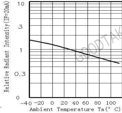
Fig. 2 Relative Radiant Intensity Vs Ambient Temperature
