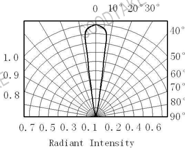
Fig.5 Angle Vs Radiant Intensity
