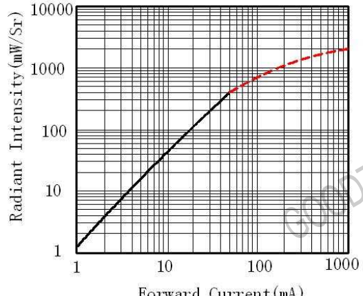
Fig.4 Forward Current Vs Radiant Intensity
