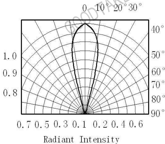
Fig.5 Angle Vs Radiant Intensity
